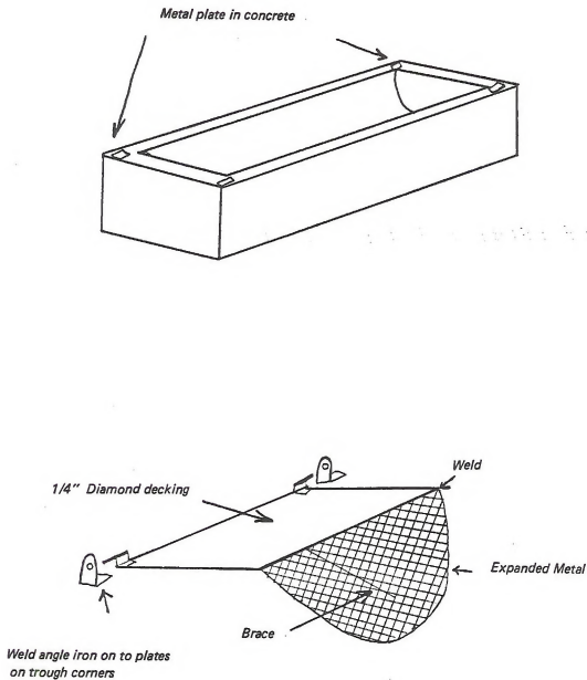
Round bottom cement trough
